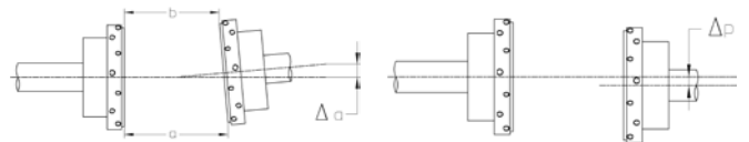
Angular Misalignment
