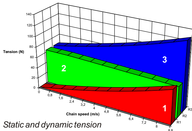
Dynamic (1), static (2) and resulting tension (3) for ROLL-RING 112 030 01
