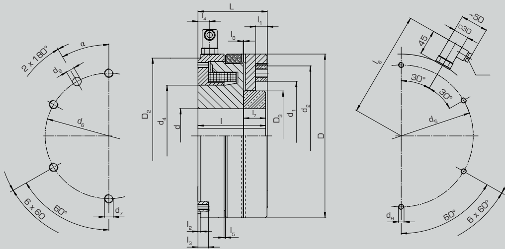
Tooth clutch with plug and socket
